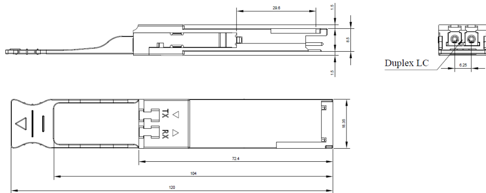
Figure 5. Mechanical Outline
